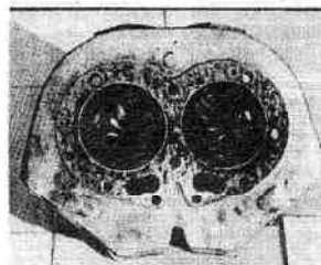
Material was removed from the intake port of stock head, not necessarily to enlarge the port, but to allow the flow of air to follow its most natural path. This can be measured on the flow bench as the instruments will fluctuate and bounce if the air becomes turbulent, indicating the path is not natural.
