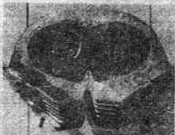
Valley Head Service increased the size of the intake valve in the stock head by .060-inch, and the exhaust measures .020-inch larger. Size and shape of valve pocket, seats, and back face of valve itself are very critical, in relation to the air flow.
