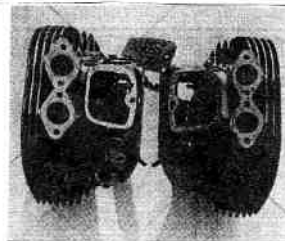
Intake side of both heads is somewhat different in modifications. Norton Road Racer (left) has had the intake ports opened up a 1/16-inch at the gasket flange, note also that passage all the way down has been enlarged and polished. Parts on the Valley Head Service one (right) haven't been opened up as large, and passageway is smaller.
