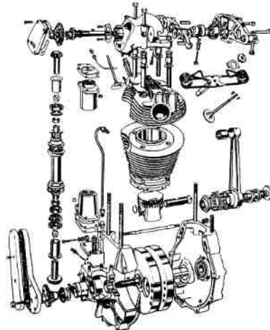
FIG. 12. An extended view of the v.t.c. engine.
