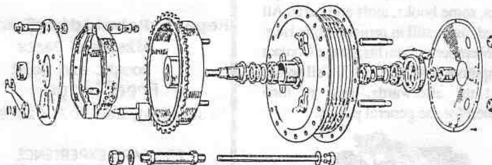
Fig. H5 1970 type rear wheel exploded
